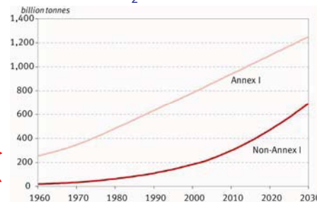
Cumulative CO 2 emissions since 1900
