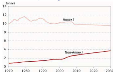
Per capita CO 2 emissions
